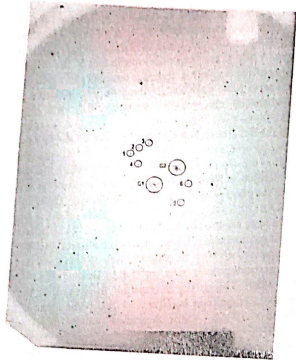
FIGURE 20. Scanned 103aO glass plate image in the field around disk galaxy with a bar NGC 5597. Six stars were selected as reference stars for astrometry, source labeled G1 and G2 are NGC 5597 and its nearby companion to the north-west disk galaxy NGC 5595. The field size and orientation is the same as in Fig. 1.
