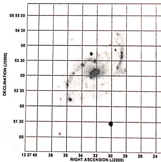
FIGURE 17. Close-up from Fig. 16 for the disk galaxy NGC 5248; grey scale is proportional to surface brightness in arbitrary units (negative image: white sky and dark bright objects). Notice the unresolved bright central region and the bright regions delineating the two spiral arms.
