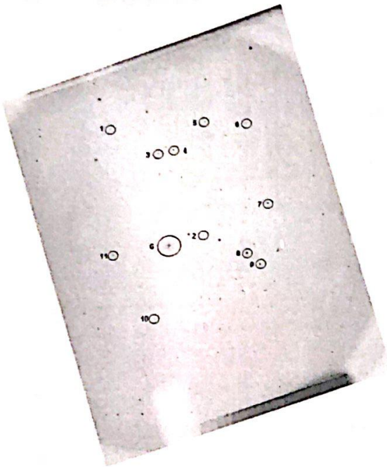
FIGURE 10. Scanned 103aO glass plate image in the field around NGC 4245. Eleven stars were selected as reference stars for astrometry, source labeled G is NGC 4245. The field size and orientation is the same as in Fig. 1.
