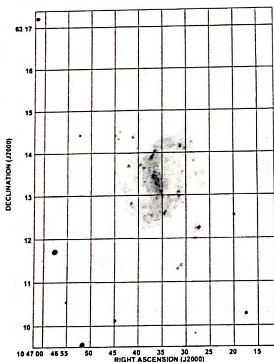
FIGURE 4. Close-up from Fig. 3 the disk galaxy with stellar bar NGC 3359; grey scale is proportional to surface brightness in arbitrary units (negative image: white sky and dark bright objects).
