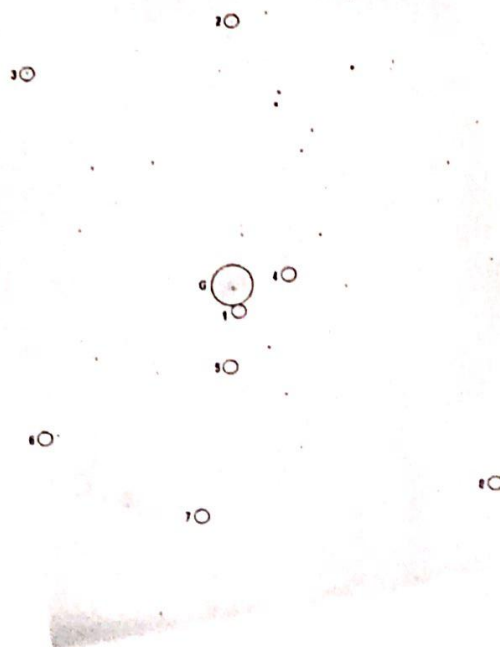
FIGURE 16. Scanned 103aO glass plate image in the field around disk galaxy NGC 5248. Eight stars were selected as reference stars for astrometry; source labeled G is NGC 5248. The field size and orientation is the same as in Fig. 1.
