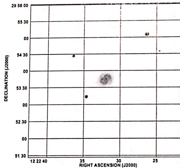
FIGURE 13. Close-up from Fig. 12 for the disk galaxy with bar NGC 4314; grey scale is proportional to surface brightness in arbitrary units (negative image: white sky and dark bright objects). This exposure shows a circumnuclear structure and a point as nucleus. Emission from the stellar bar is weak and no emission was detected from the spiral arms.
