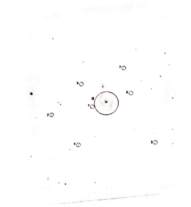
FIGURE 14. Scanned 103aO glass plate image in the field around disk galaxy NGC 5194 (M51). Seven stars were selected as reference stars for astrometry; source labeled G is NGC 5194 with its companion NGC 5195 to its north. The field size and orientation is the same as in Fig. 1.
