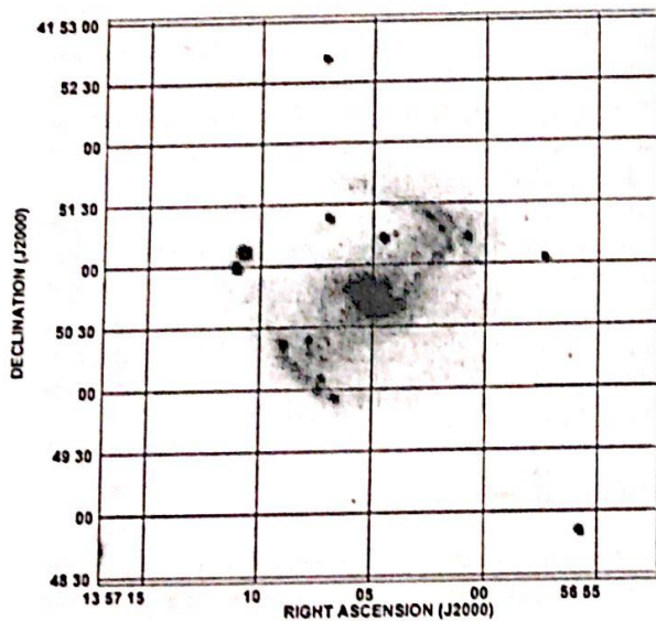
FIGURE 19. Close-up from Fig. 18 for the disk galaxy with a bar NGC 5383; grey scale is proportional to surface brightness in arbitrary units (negative image: white sky and dark bright objects). Notice the low surface brightness almost at the center of the bar and the bright central region.
