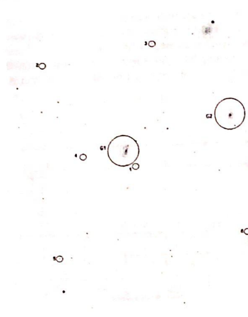
FIGURE 5. Scanned 103aO glass plate image in the field around disk galaxy NGC 3627. Six stars were selected as reference stars for astrometry, labeled 1 through 6; sources labeled G1 and G2 are the disk galaxies NGC 3627 and its nearby companion NGC 3623 respectively. The field size and orientation is the same as in Fig. 1.
