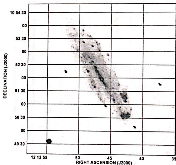
FIGURE 9. Close-up from Fig. 8 for the disk galaxies NGC 4178; grey scale is proportional to surface brightness in arbitrary units (negative image: white sky and dark bright objects). Notice the bright sources to the south-west.
