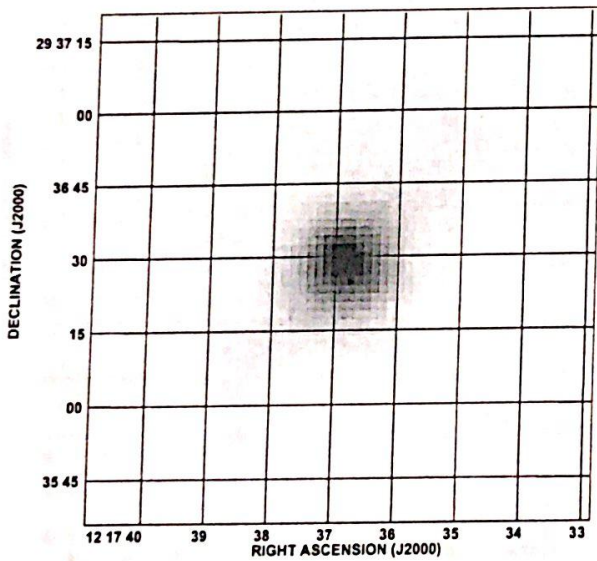
FIGURE 11. Close-up from Fig. 10 for NGC 4245; grey scale is proportional to surface brightness in arbitrary units (negative image: white sky and dark bright objects). This image shows a bright nucleus and weak emission from the disk.
