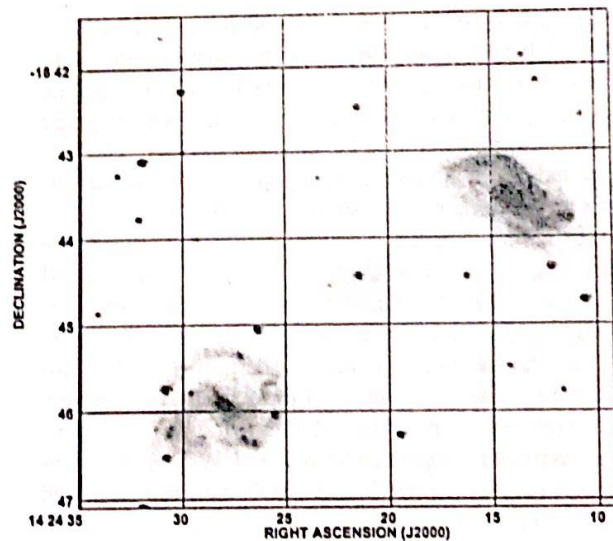
FIGURE 21. Close-up from Fig. 20 for the disk galaxy with a bar NGC 5597 (lower left on the image) and its nearby companion disk galaxy NGC 5595 (upper right on the image, north-west side of NGC 5597); grey scale is proportional to surface brightness in arbitrary units (negative image: white sky and dark bright objects). Notice the spiral arms in NGC 5597 facing NGC 5595; its spatial position might suggest a tidal interaction. NGC 5595 is the only large-scale companion of NGC 5597 within 20 diameters [11].
