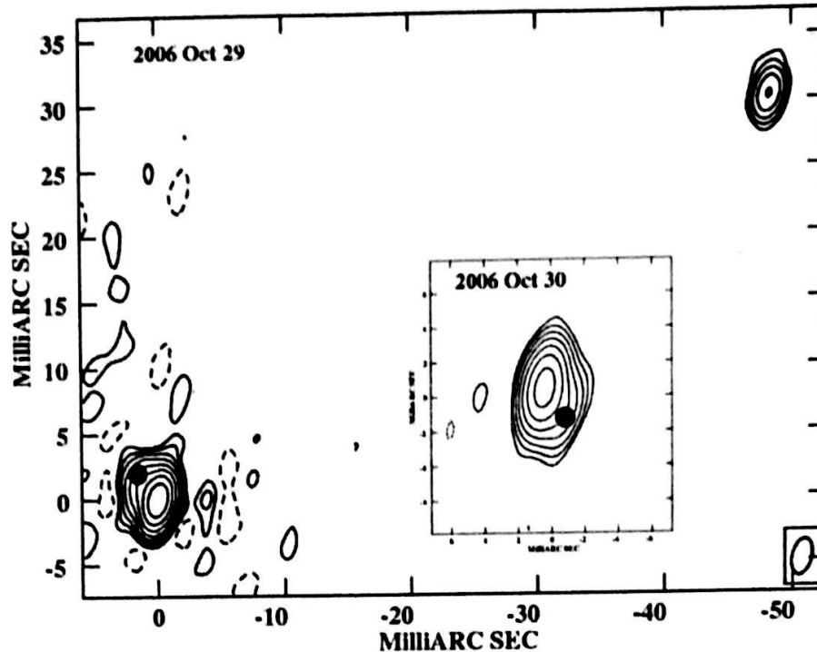
Figure 1. An image of the Algol triple system made from the NPOI data of 2006 Oct 29. Algol C is the component in the upper right hand corner. The insert shows a close-up image made from the NPOI observation of 30 Oct 2006 and emphasizes the motion of Algol B between the two epochs. To guide the eye, the approximate positions of Algol B are indicated at each epoch by a filled black circle. All figures are from Zavala et al. (2010).
