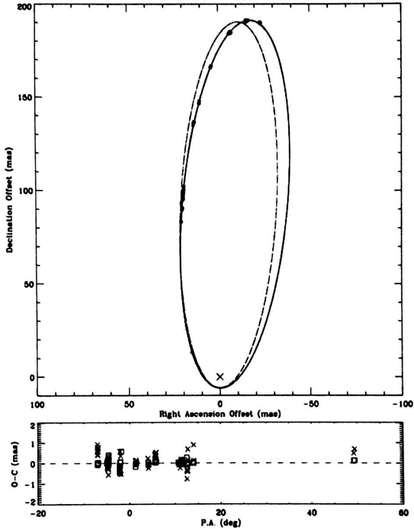
Figure 4. Top: Plot of data for \delta Sco. The figure shows the relative visual orbit of the system; the x and y scales are in milliarcseconds. NPOI measurements are shown as solid circles, with the corresponding best-fit orbit shown as a solid curve. The dashed curve represents the best orbit from Tango et al. (2009). The uncertainty ellipses of the NPOI data are generally smaller than the size of the plotted symbols. The location of the primary is marked with a cross. Bottom: The east-west (squares) and north-south (crosses) components of the O-C vectors as a function of the P.A. of the secondary.
